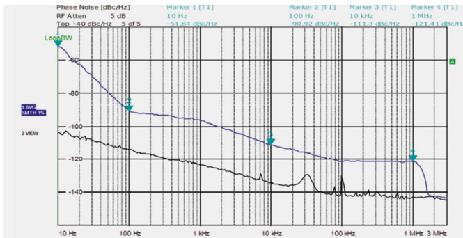
Figure 10: Phase noise simulation for HD radio AM
