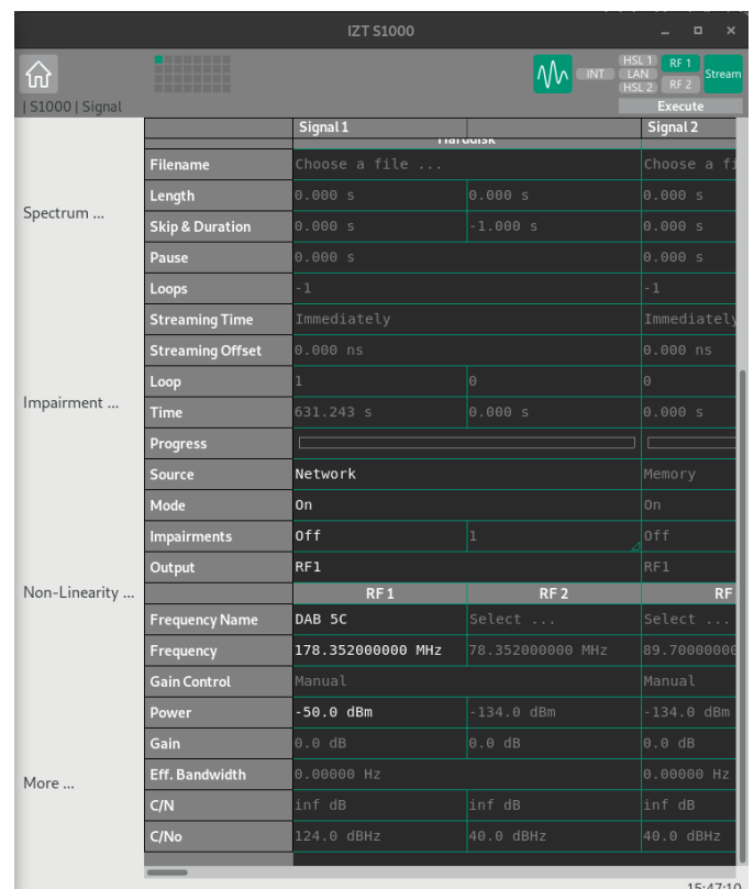
Figure 21: DAB EDI modulator
