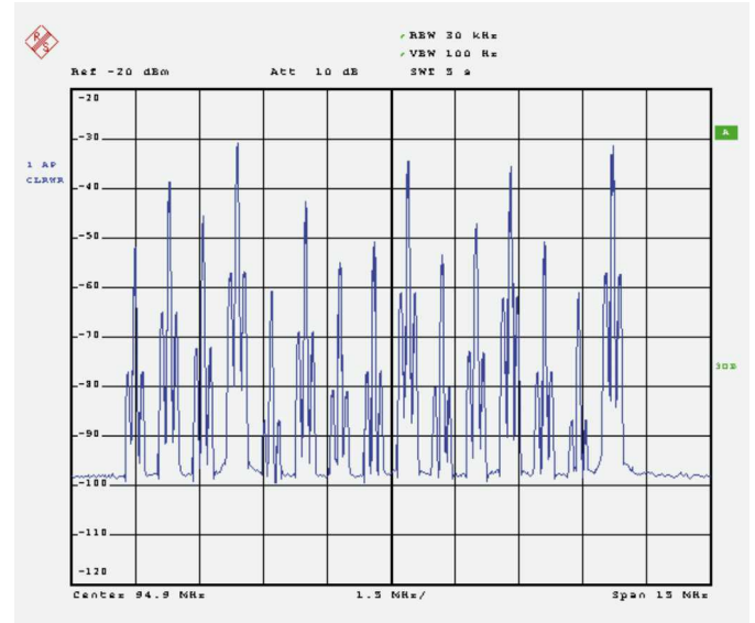
Figure 23: 15 HD radio signals
