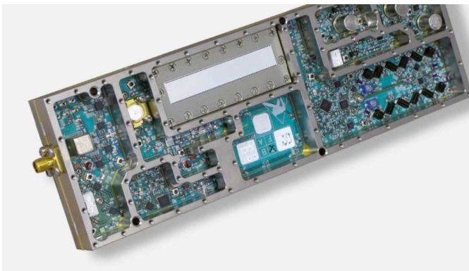
Figure 3: RF section of the S1000
