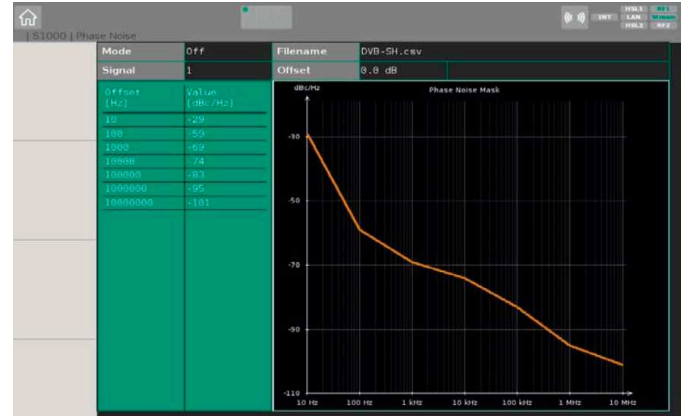
Figure 11: Phase noise configuration
