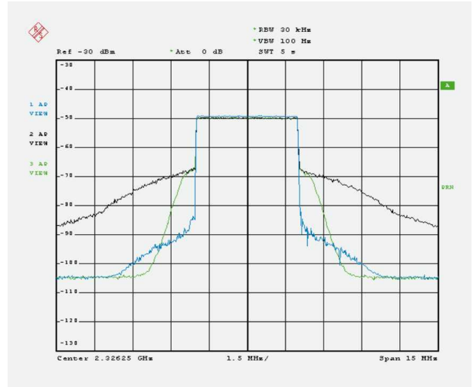
Figure 8: Distorted signal before (black), after filter simulation (green), and after filter simulation with alternative filter settings (blue)
