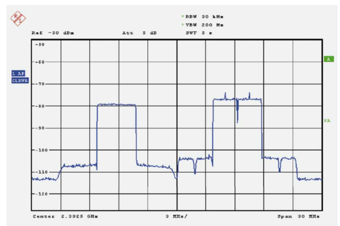
Figure 24: SIRIUS XM radio signal using 8 VSG
