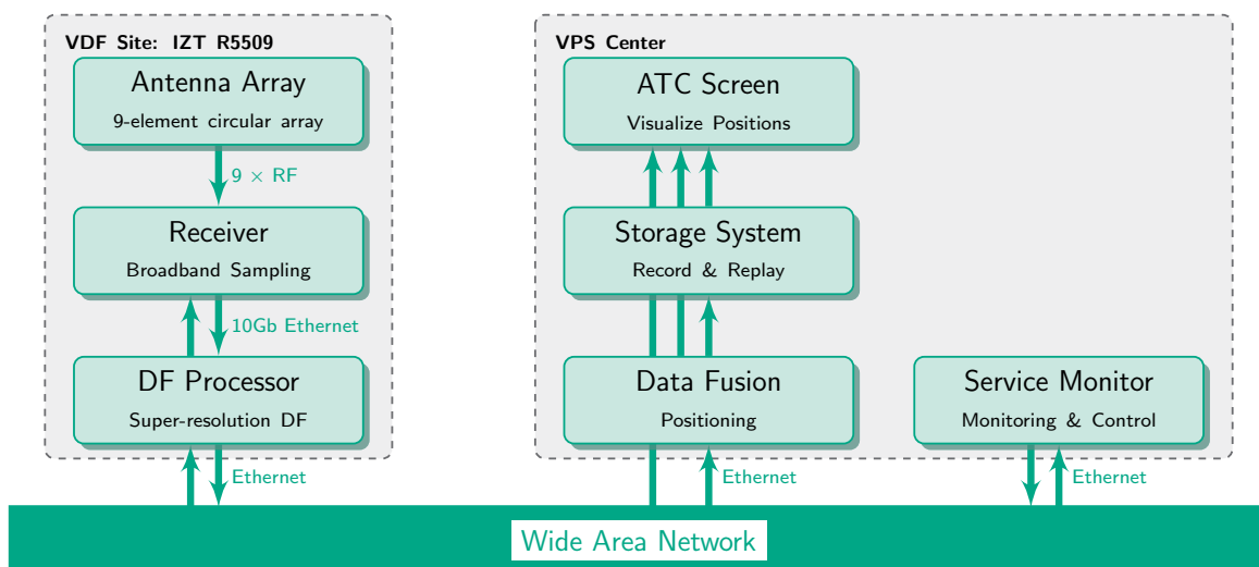
FIGURE 9: HIGH LEVEL ARCHITECTURE OF A VPS SYSTEM
