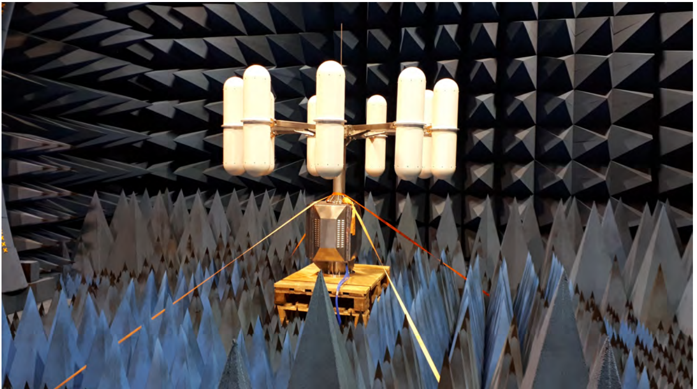
FIGURE 5: MEASUREMENT OF THE 9-ELEMENT PROTOTYPE ANTENNA
