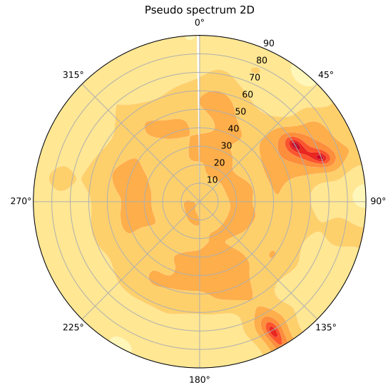
FIGURE 6: 2D MUSIC SPECTRUM FOR 3 SIGNAL SOURCES ON THE SAME FREQUENCY AT AZIMUTHS AND ELEVATIONS OF 60°, 70°, 150° AND 30°, 20°, 10°, RESPECTIVELY
