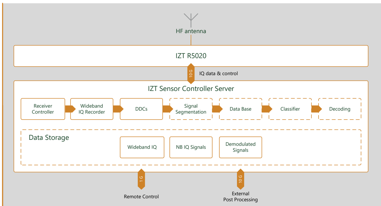
Figure 5: IZT R5020 WITH IZT SENSOR CONTROLLER PC
