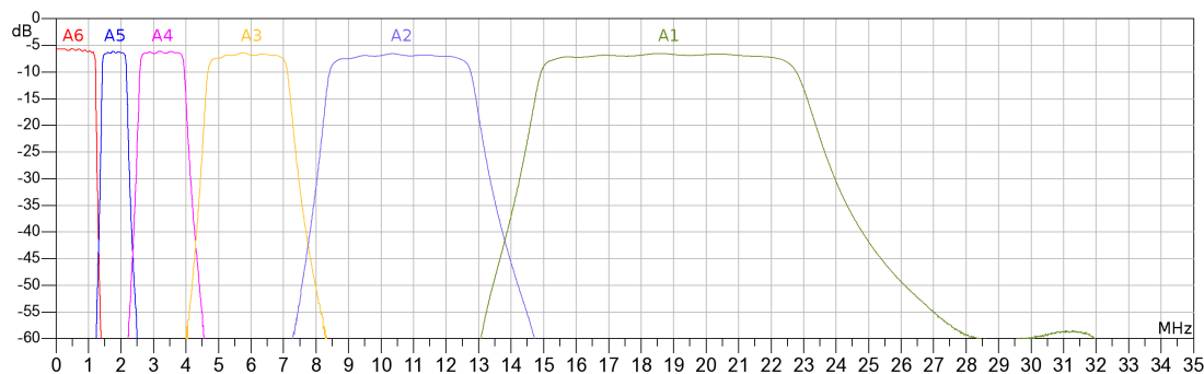
Figure 3: IZT R5020 BAND-PASS FREQUENCY RESPONSE OF FILTER BANK A
