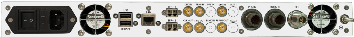
Figure 7: IZT R5020 REAR PANEL
