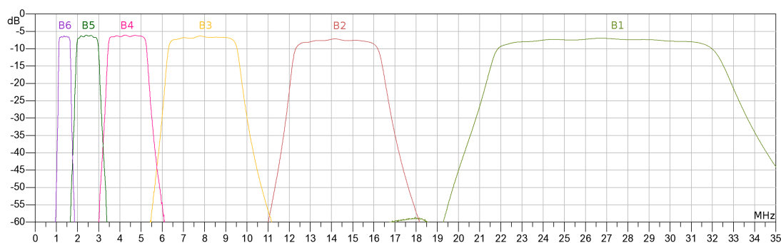
Figure 4: IZT R5020 BAND-PASS FREQUENCY RESPONSE OF FILTER BANK B
