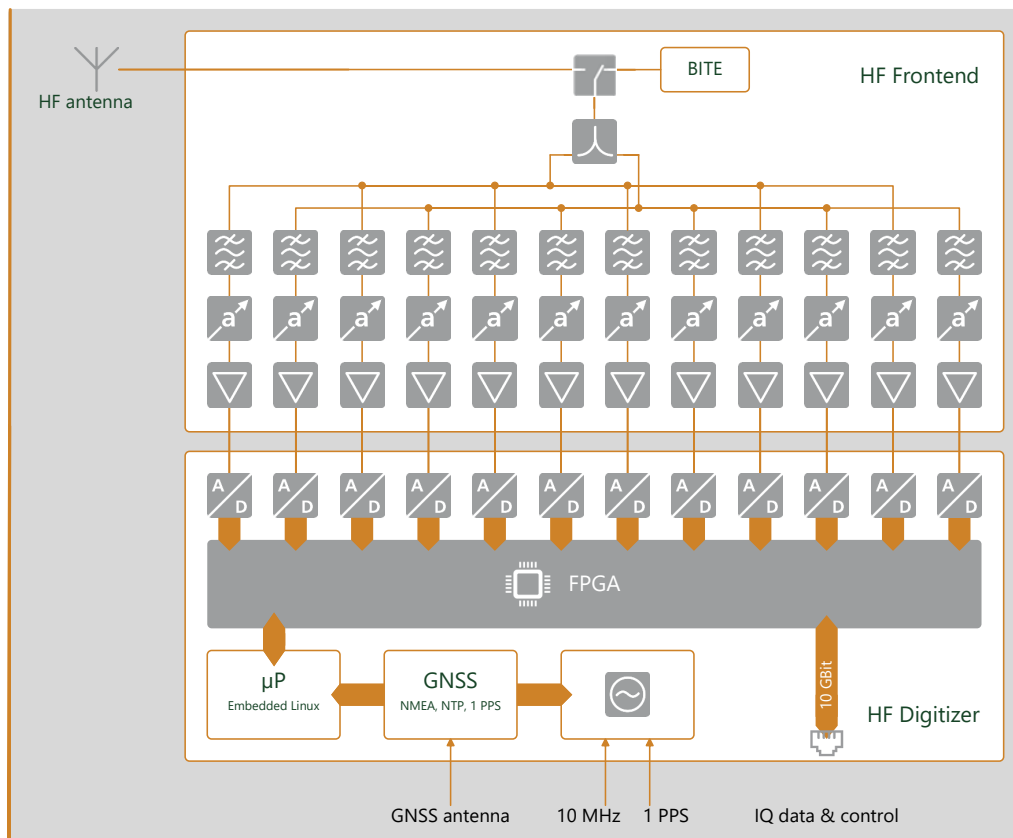
Figure 2: IZT R5020 BLOCK DIAGRAM
