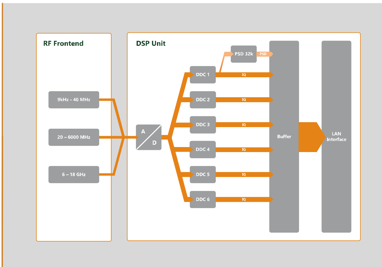
Figure 3: IZT R5010 Receiver Block Diagram
