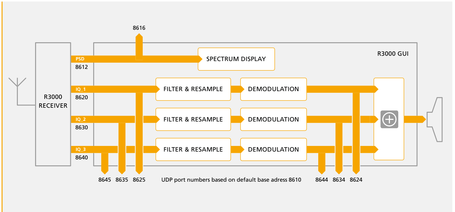
FIGURE 7: UDP PORTS OF R3000 GUI AVAILABLE FOR REMOTE APPLICATIONS
