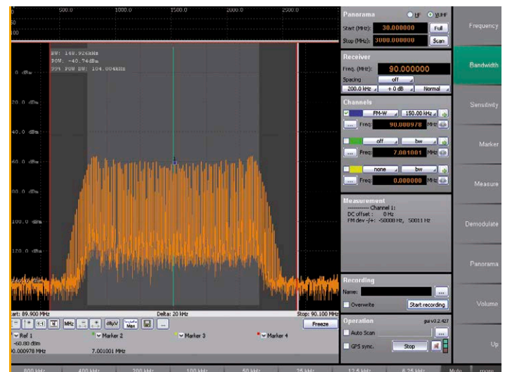
FIGURE 4: FM MODULATION AND OCCUPANCY MEASUREMENT
