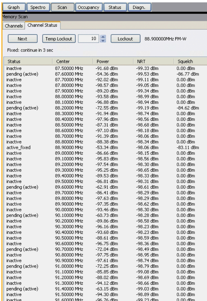
FIGURE 6: CHANNEL STATUS INFORMATION DURING A SCAN
