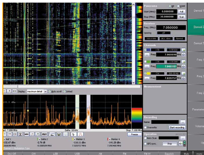
FIGURE 1: COMBINED SPECTRUM AND WATERFALL DISPLAY
