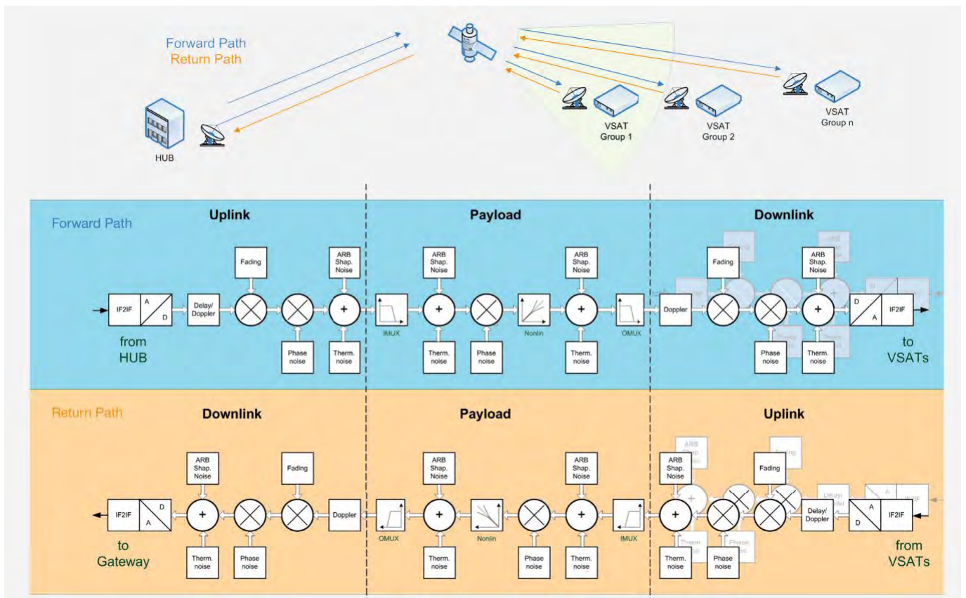
FIGURE 1: CHANNEL AND PAYLOAD MODELS OF IZT C6000
