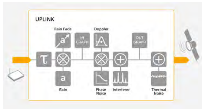
FIGURE 3: BLOCKDIAGRAM OF UPLINK EFFECTS
