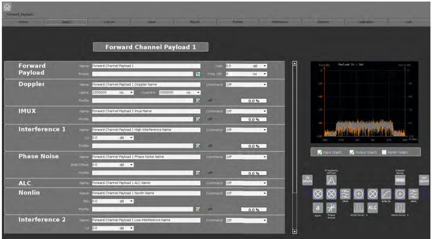
FIGURE 8: PAYLOAD CONFIGURATION
