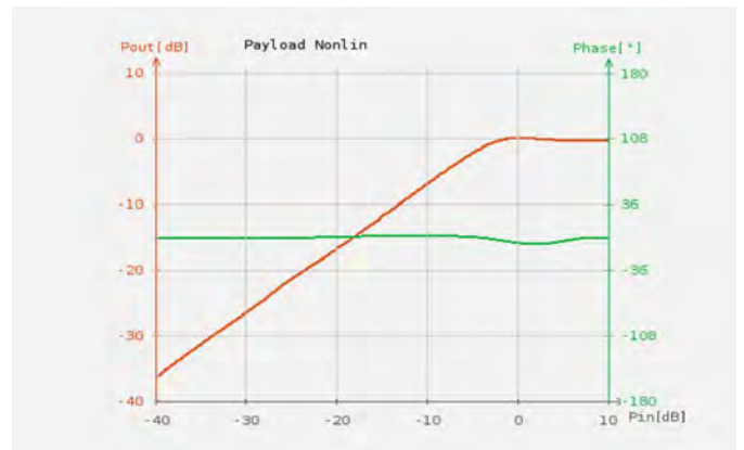
FIGURE 7: LTWTA CURVE: AM/AM AND PHASE VERSUS IBO DISTORTION
