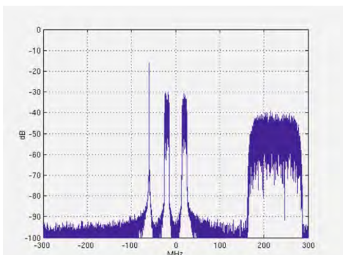
FIGURE 9: EXAMPLE OF AN INTERFERER SCENARIO
