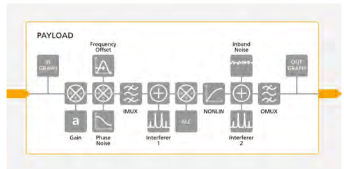
FIGURE 6: BLOCKDIAGRAM OF PAYLOAD EFFECTS
