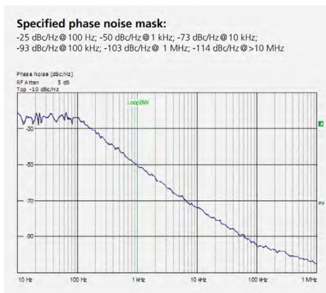
FIGURE 5: SIMULATED PHASE NOISE "DVB-S2 TYPICAL"
